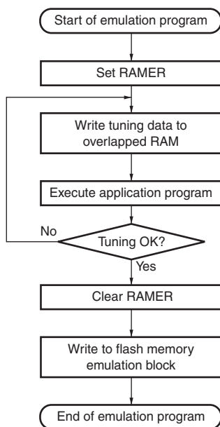
Figure 19.7 Flowchart for Flash Memory Emulation in RAM
