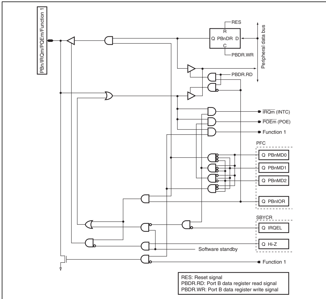
Figure D.15 \overline{\text{PBn/IRQm/POEm/Function 1}}
