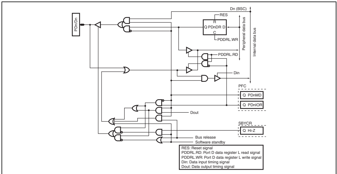
Figure D.23 PDn/Dn
