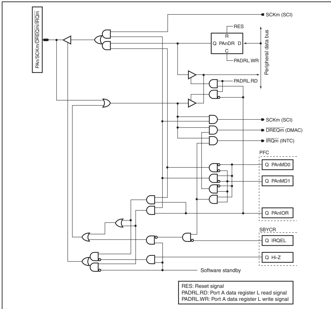
Figure D.3 PAn/SCKm/ \overline{\text{DREQm}} / \overline{\text{IRQm}}
