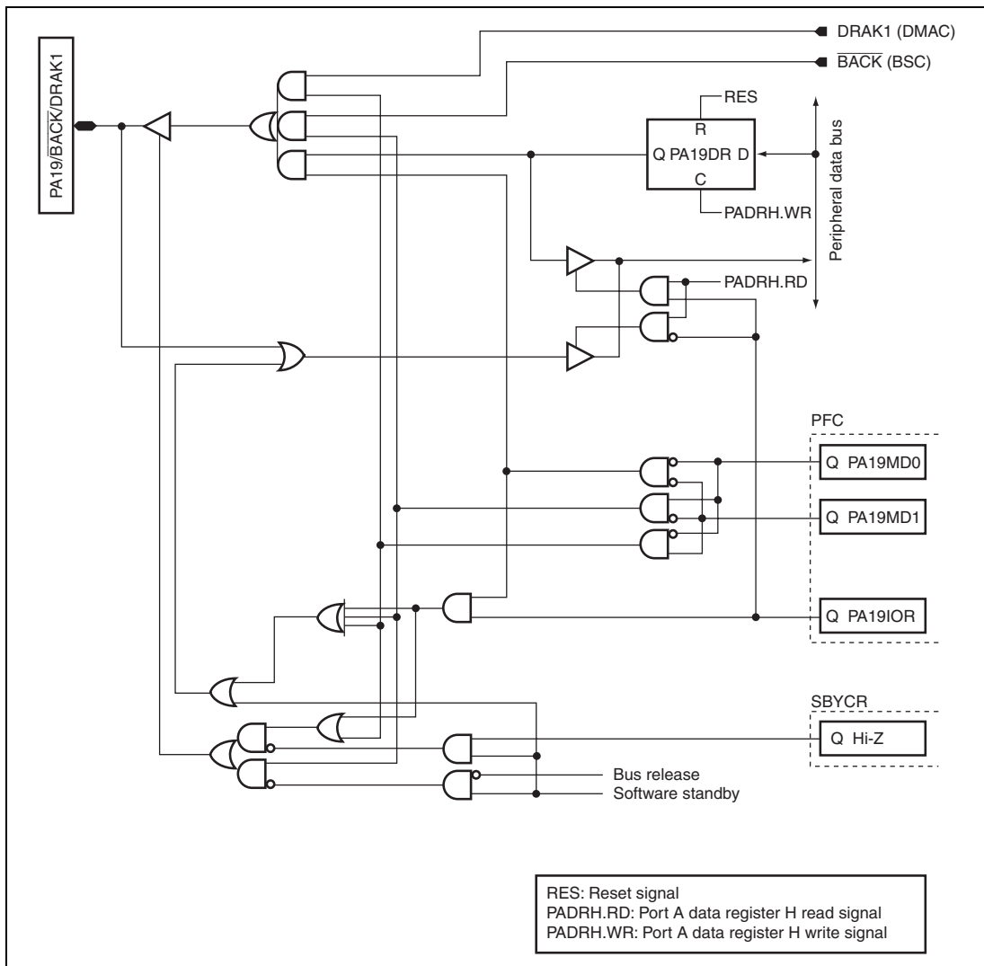
Figure D.11 PA19/ \overline{\text{BACK}} /DRAK1
