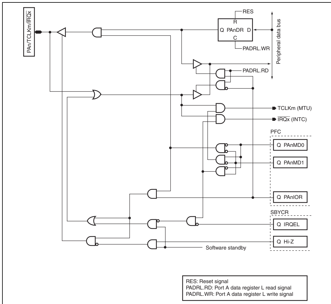
Figure D.5 PAn/TCLKm/ \overline{\text{TRQx}}
